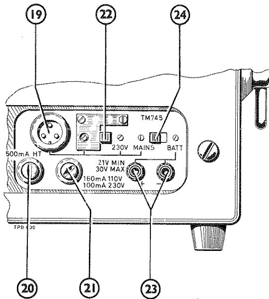
Fig. 2.3 Rear panel
